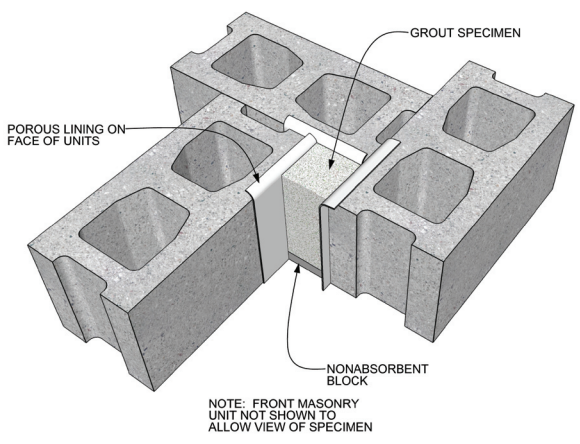
MOLD FOR UNITS OVER 6" IN HEIGHT
