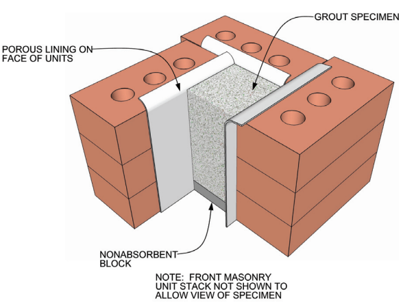
MOLD FOR UNITS 6" OR LESS IN HEIGHT
