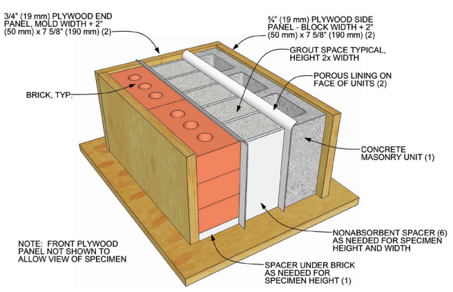
MOLD FOR COMBINATIONS OF UNITS
