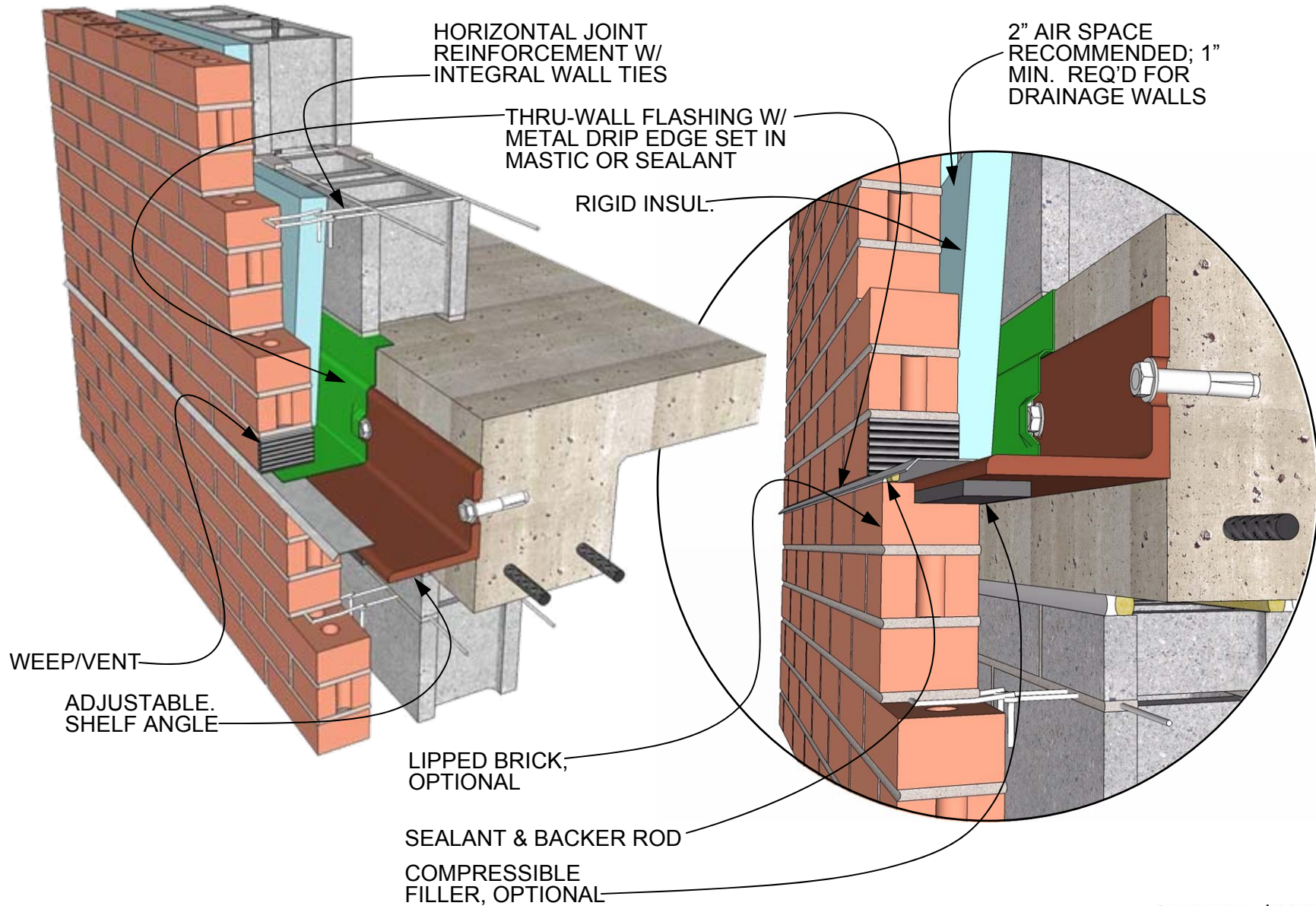
SHELF ANGLE DETAIL LIPPED BRICK DETAIL 01.030.0702 REV. 10/14/07
